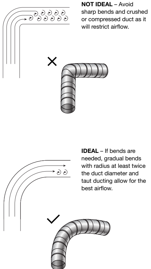
Diagram 2: DUCT BENDS
