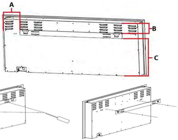
SPS-50/60/74B-AU Wall Bracket Illustrated
