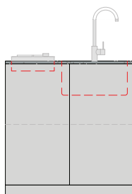
AC9002D-WOK-ST 900mm | 2 Doors | Wok Burner Sink & Tap
